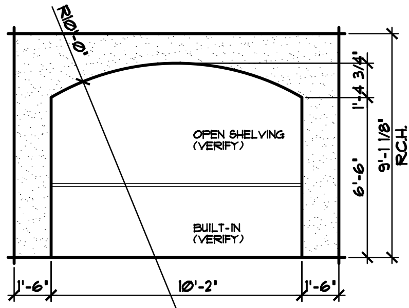
① FIREPLACE ELEVATION VIEW FROM LIVING ROOM 1/4"=1'-0"
